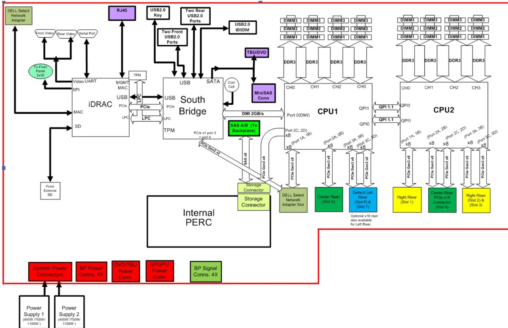
Figure 19. R720 system board block diagram
