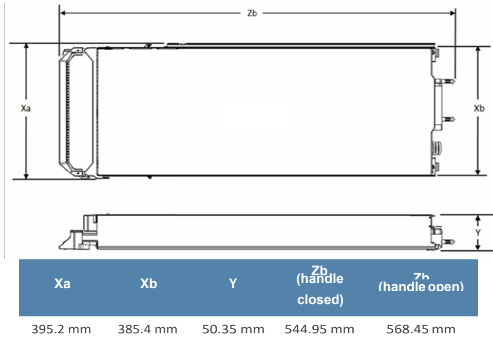
Figure 8. Module dimensions
