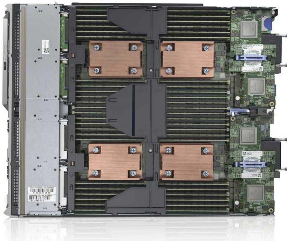
Figure 3. M820 internal module view
