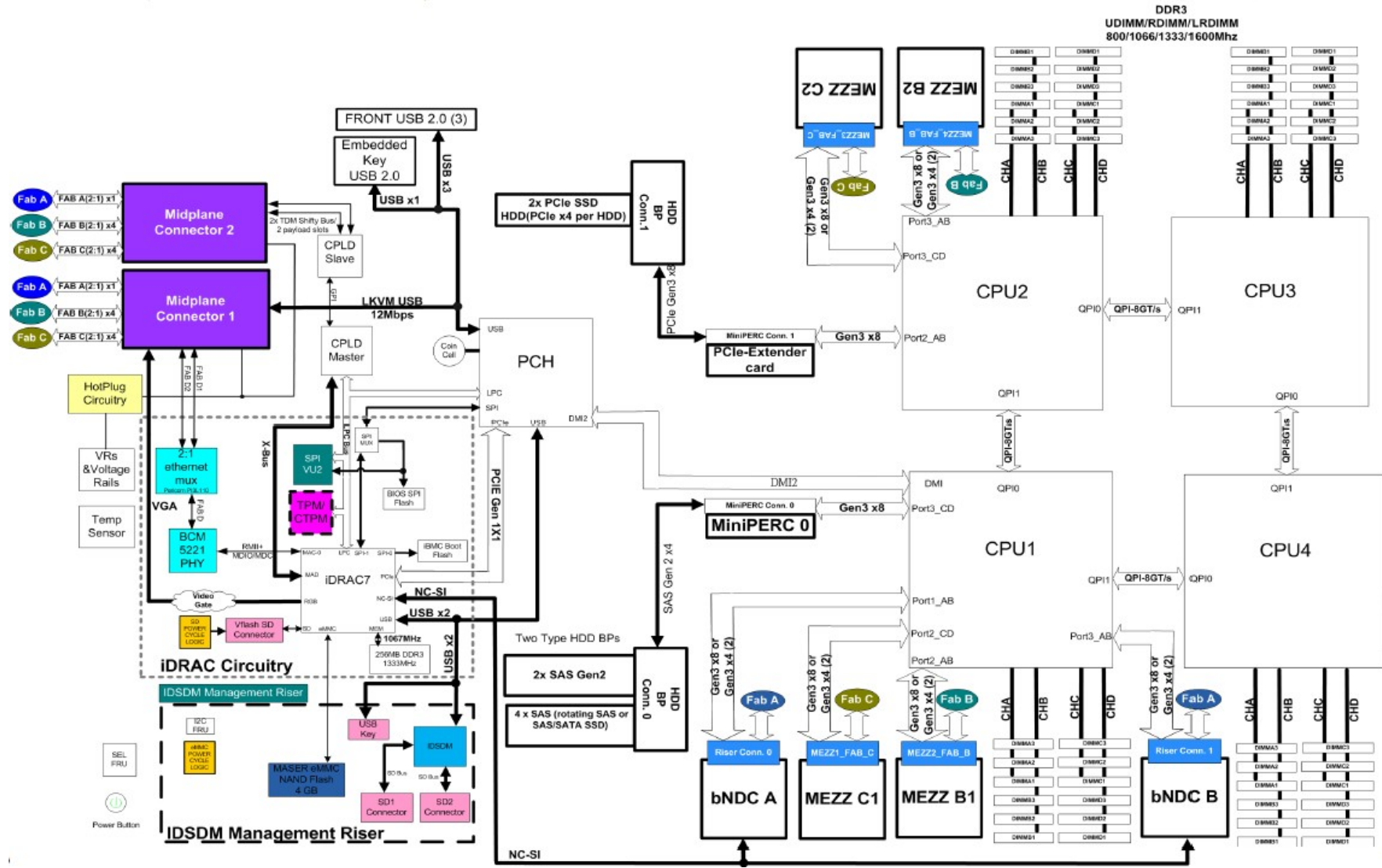
Figure 9. M820 system board block diagram
