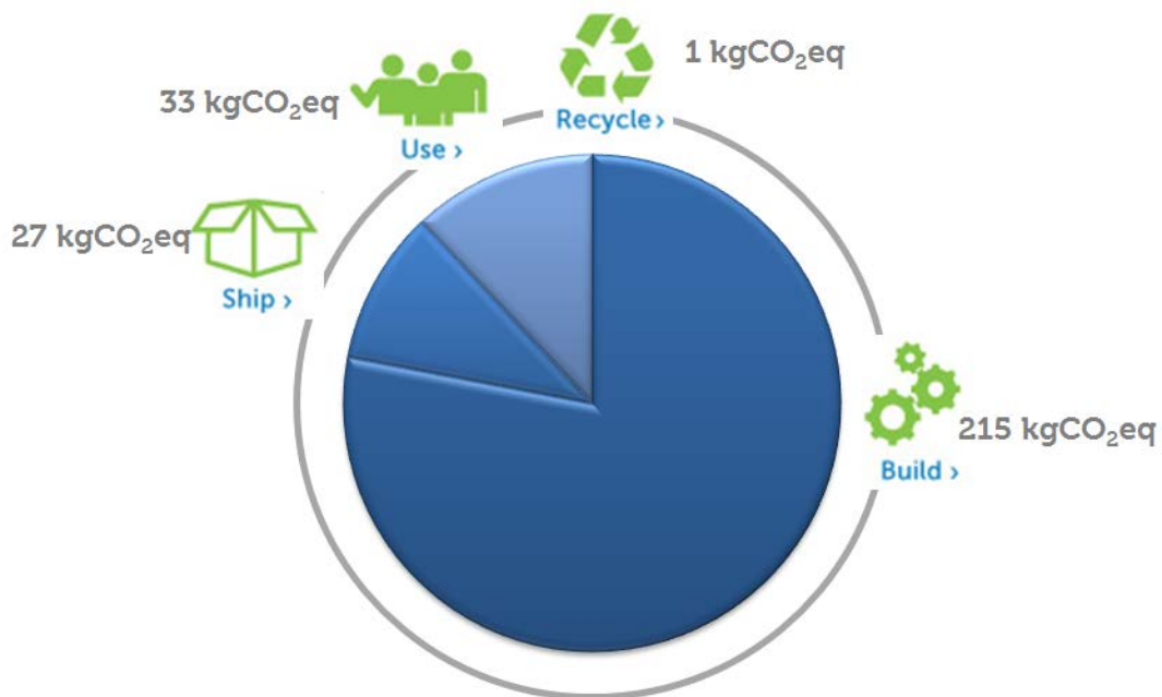
Figure 2: Total Product Carbon Footprint [kgCO 2 eq] of the Latitude E7440 Laptop in the US.
