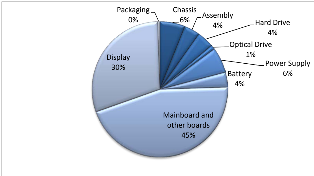
Figure 3: Breakdown of manufacturing phase in the carbon footprint. Total manufacturing contribution is 225 kgCO 2 eq, or 77% of the total carbon footprint.
