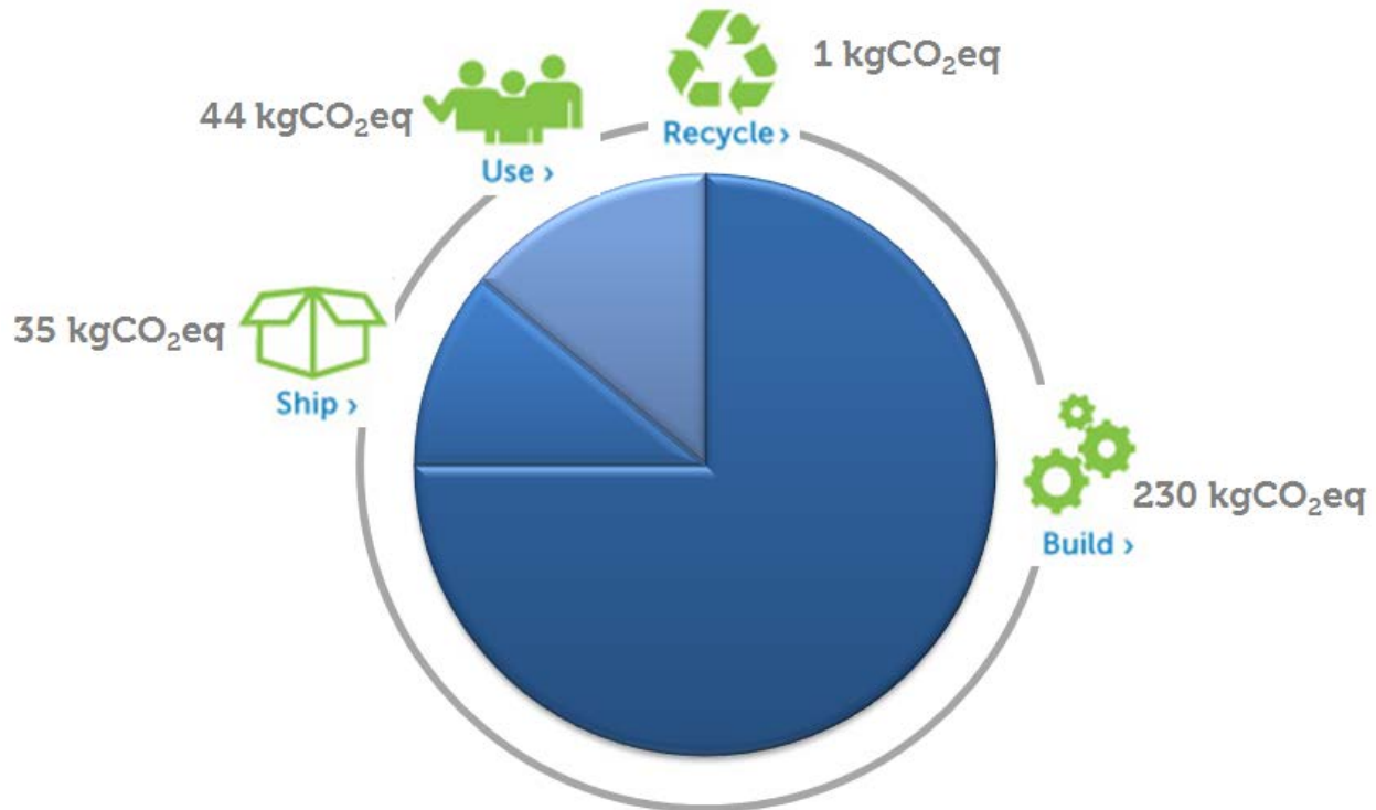
Figure 2: Total Product Carbon Footprint [kgCO 2 eq] of the Latitude E3540 Laptop in the US.
