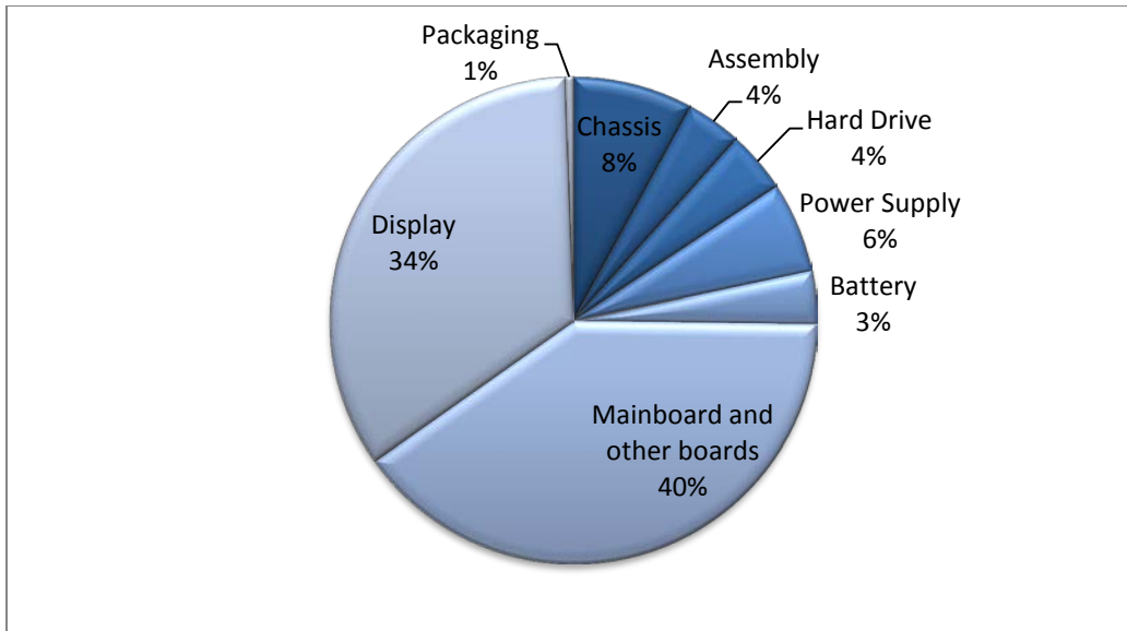
Figure 3: Breakdown of manufacturing phase in the carbon footprint. Total manufacturing contribution is 230 kgCO 2 eq, or 75% of the total carbon footprint.
