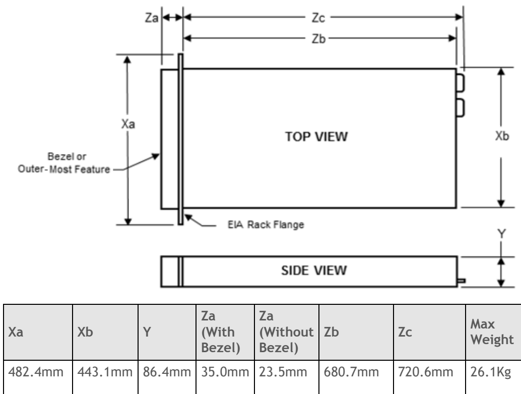
Figure 1. Chassis Dimensions
