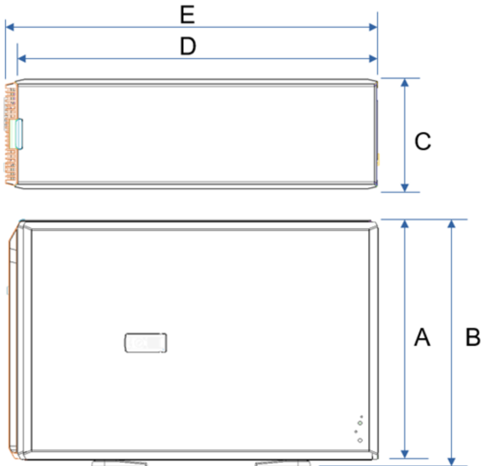
Figure 16. Chassis dimensions
