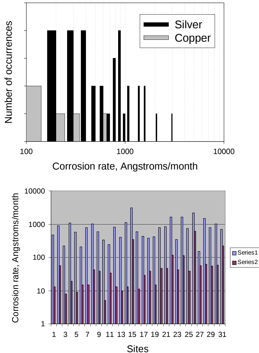
Figure 4 : IT equipment fails in data centers with reported copper creep corrosion and/or silver corrosion. The copper corrosion rate average and standard deviation was 71 and 121 C/month. . The silver corrosion rate average and standard deviation was 848 and 641 C/month. Series 1 refers to silver corrosion and series 2 to copper. Notice that in these 31 sites with known hardware failures due to corrosion, the silver corrosion rate was typically an order of magnitude or more greater than the copper corrosion rate.
