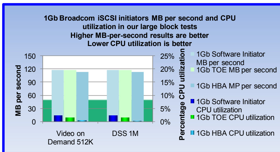
Figure 1: Average CPU utilization and MB-per-second results in our large block tests for the Broadcom NIC using a Software Initiator, TOE, and HBA. The solid green background represents 8 percent CPU usage.
