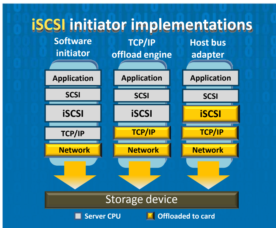
Figure 5: Three types of iSCSI initiator implementations.
