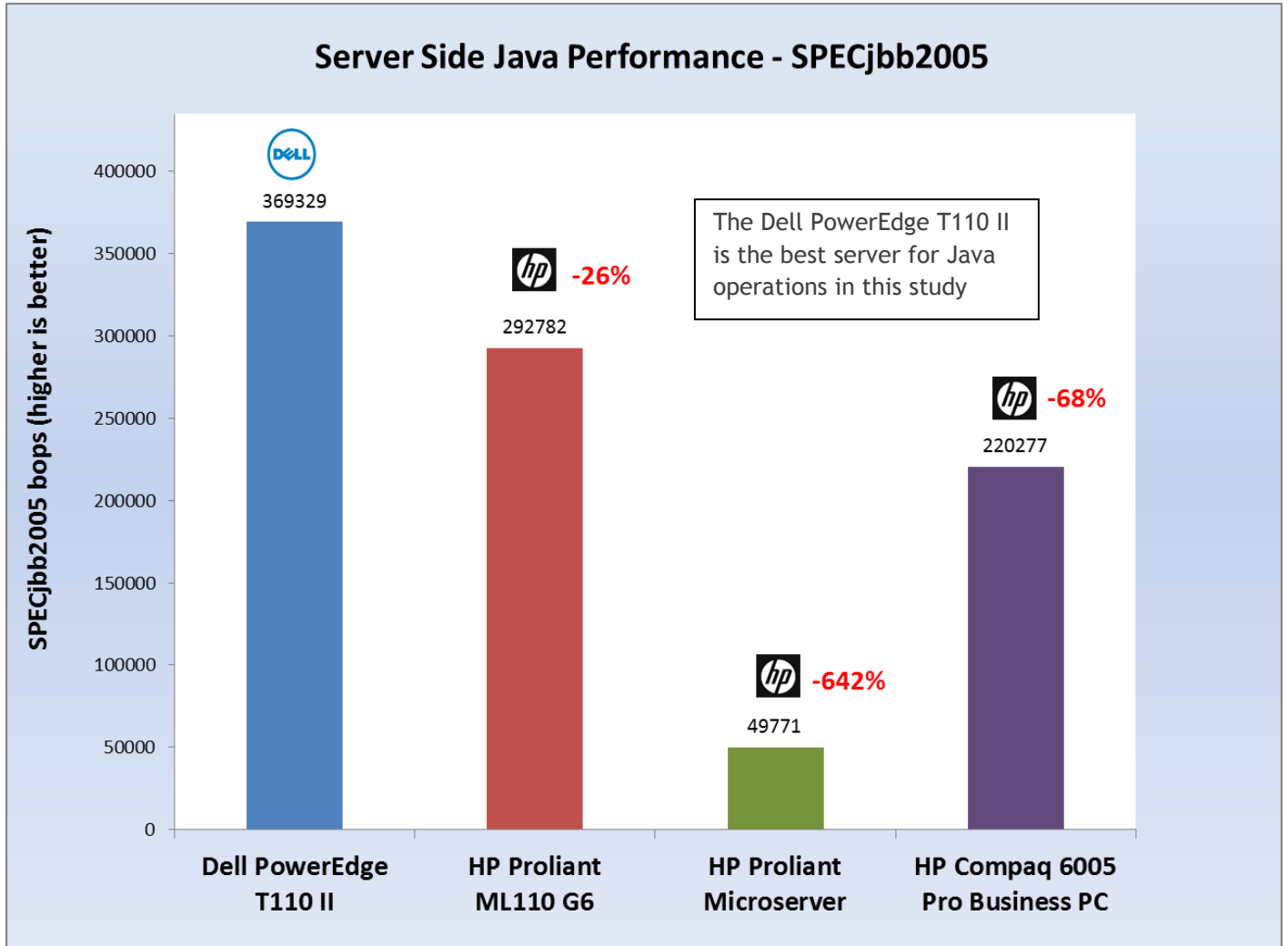
Figure 2: Comparison 1 - Processor Performance - SPECjbb2005 benchmark
