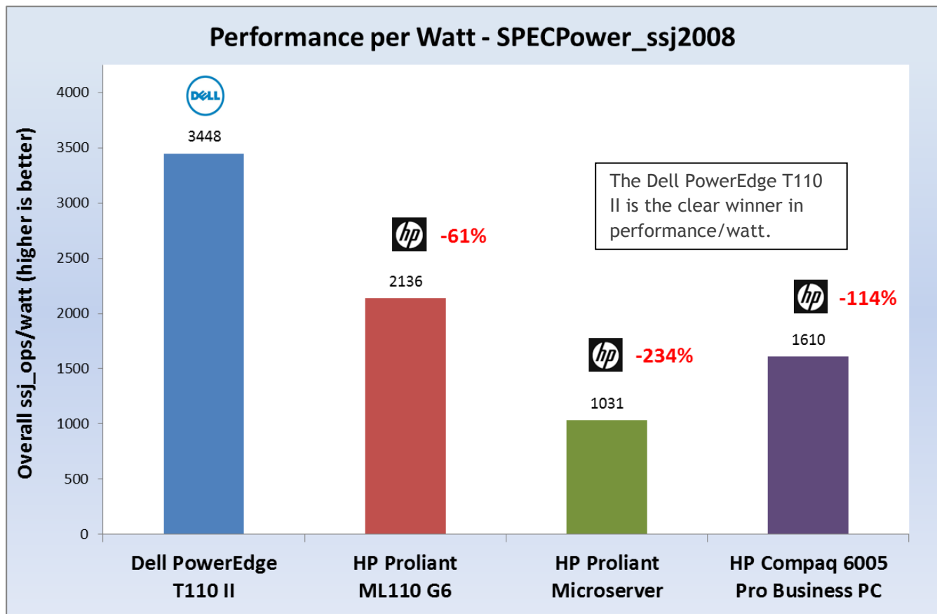
Figure 4: Comparison 3 - SPECpower_ssj2008 Overall Performance per Watt (ssj_ops/watt)
