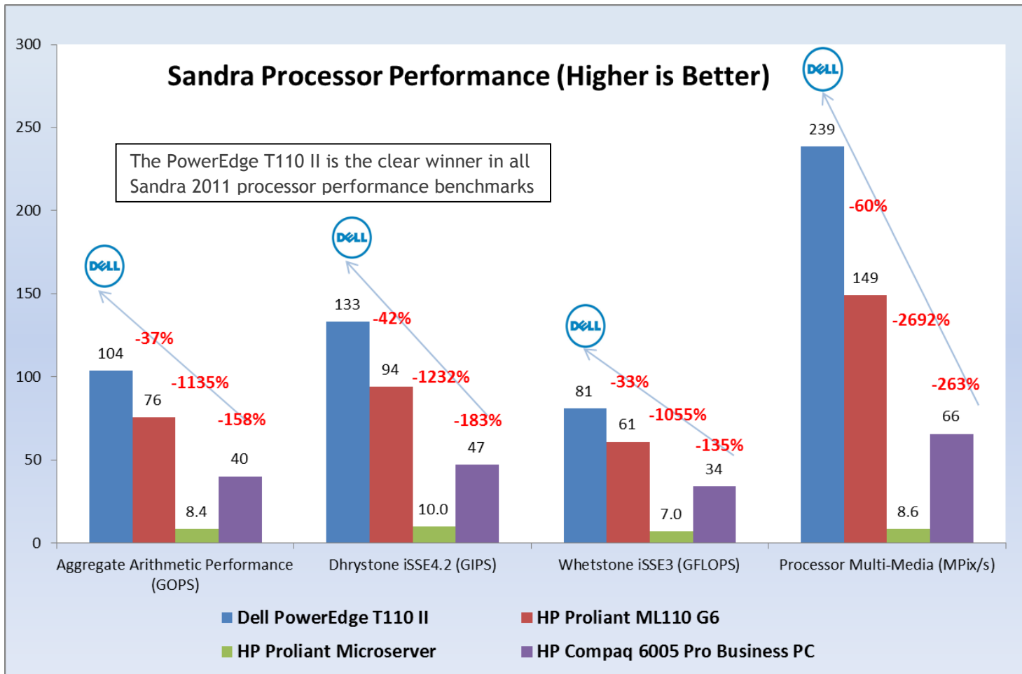
Figure 1: Comparison 1 - Sandra 2011 SP2b Processor Performance Benchmarks
