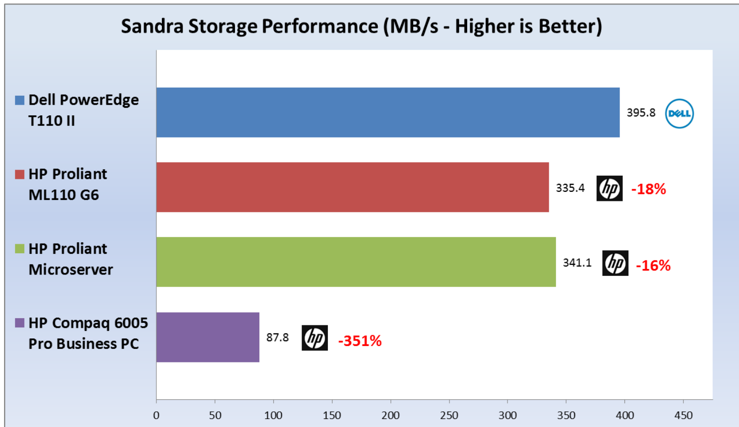
Figure 5: Comparison 4 Sandra 2011 Storage Subsystem Performance
