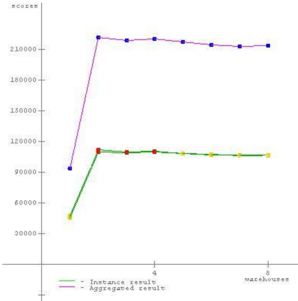
Figure 9: Comparison 1 - SPECjbb2005 Results for HP Compaq 6005 Pro Business PC
