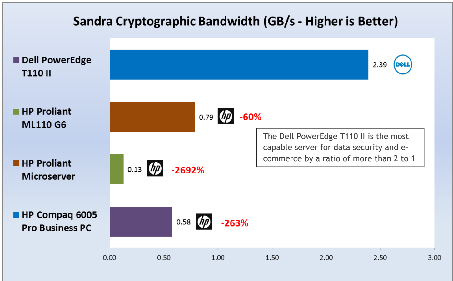
Figure 3: Comparison 2 - SiSoftware Sandra 2011 Cryptographic Bandwidth (Gb/s)
