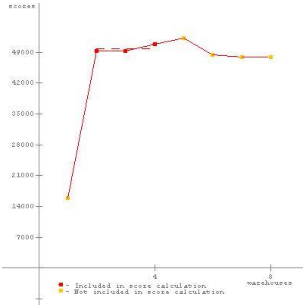
Figure 8: Comparison 1 - SPECjbb2005 Results for HP Proliant Microserver
