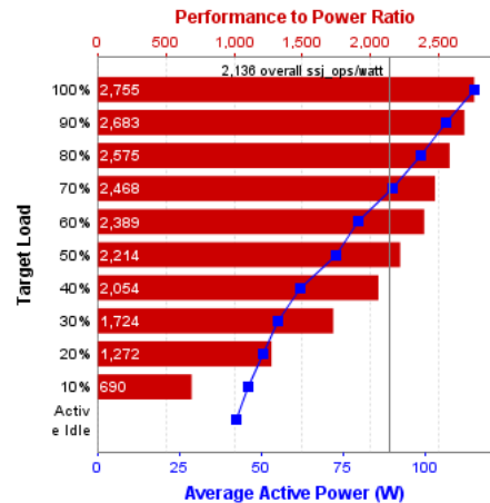
Figure 12: Comparison 3 - SPECpower_ssj2008 Results for HP Microserver
