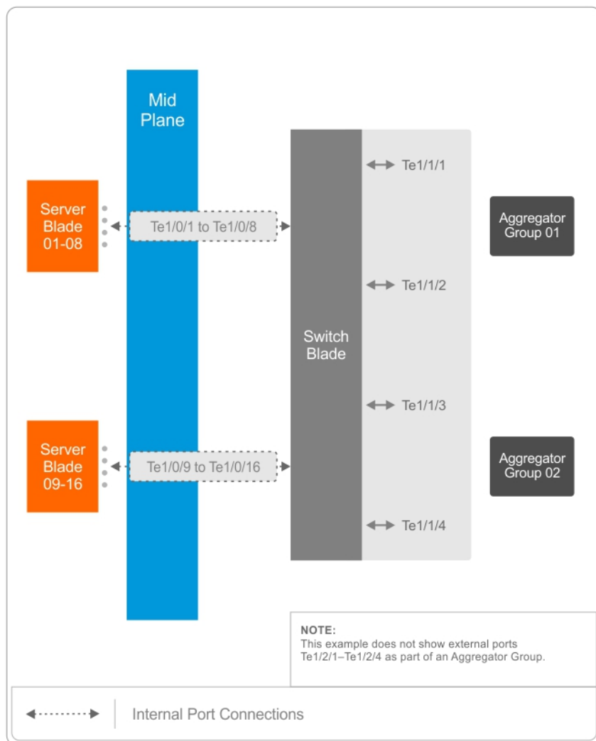
Figure 9. Single M8024 Switch Configuration with Two Aggregator Groups
