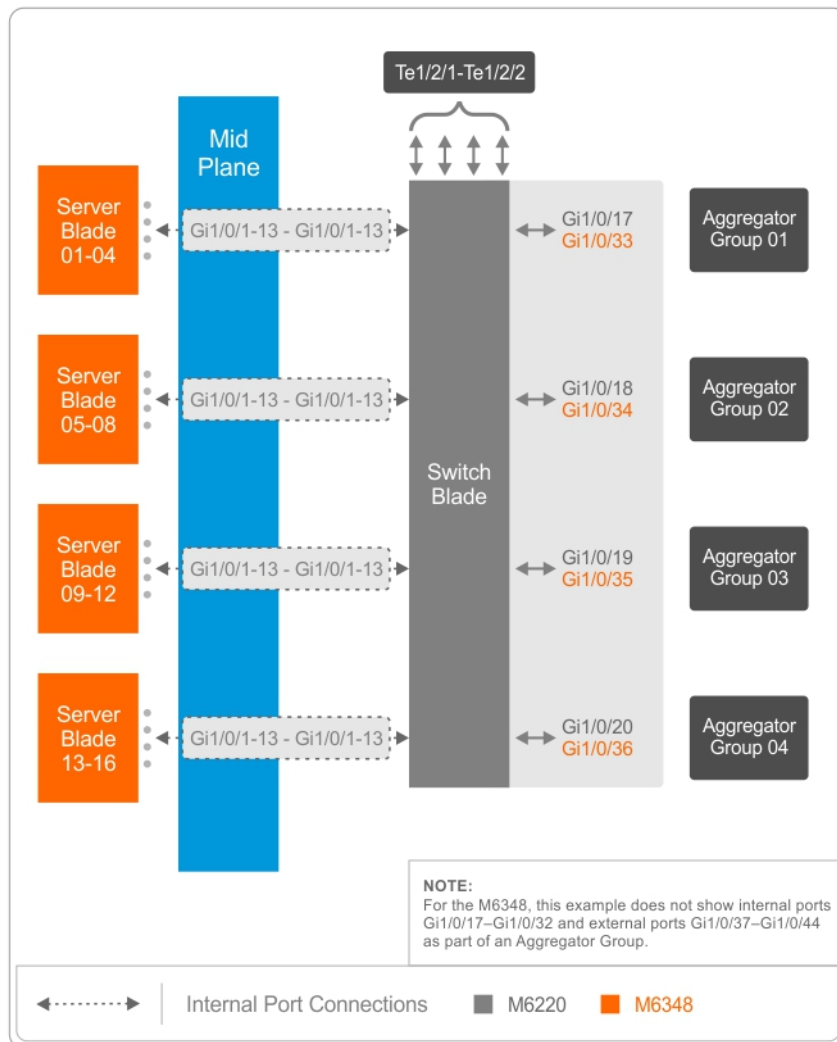
Figure 4. Single M6220/M6348 Switch with Four Aggregator Groups — Each Having Single Uplink
