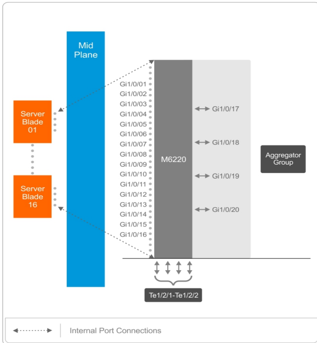
Figure 1. Default Aggregator Groups on a Modular Switch
