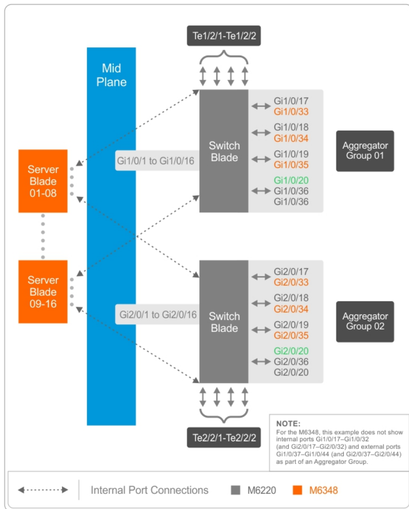
Figure 10. Stacked M6220/M6348 Switch Configuration with Two Aggregator Groups — Each Having Four Uplinks
