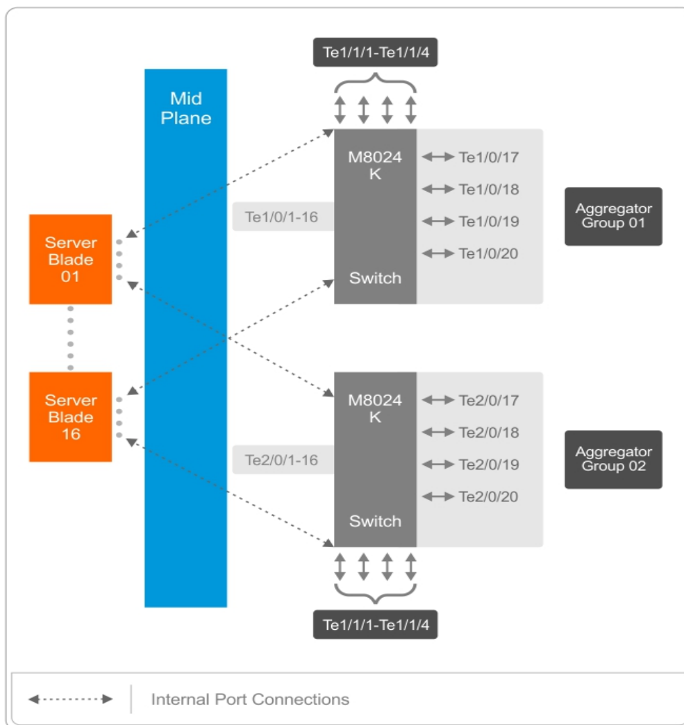
Figure 2. Default Aggregator Groups on a Stack of Two M8024K Switches
