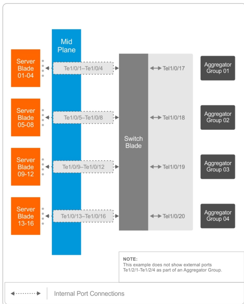
Figure 6. Single M8024K Switch with Four Aggregator Groups — Each Having Single Uplink
