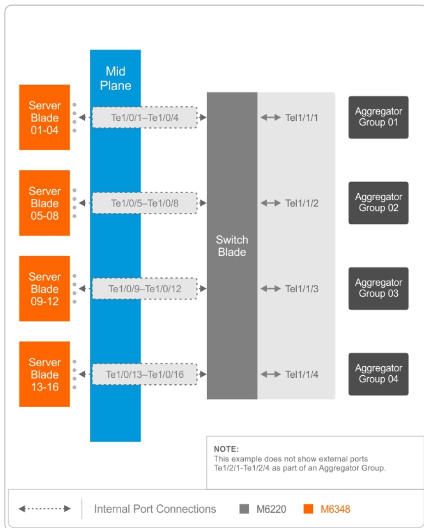
Figure 5. Single M8024 Switch with Four Aggregator Groups — Each Having Single Uplink
