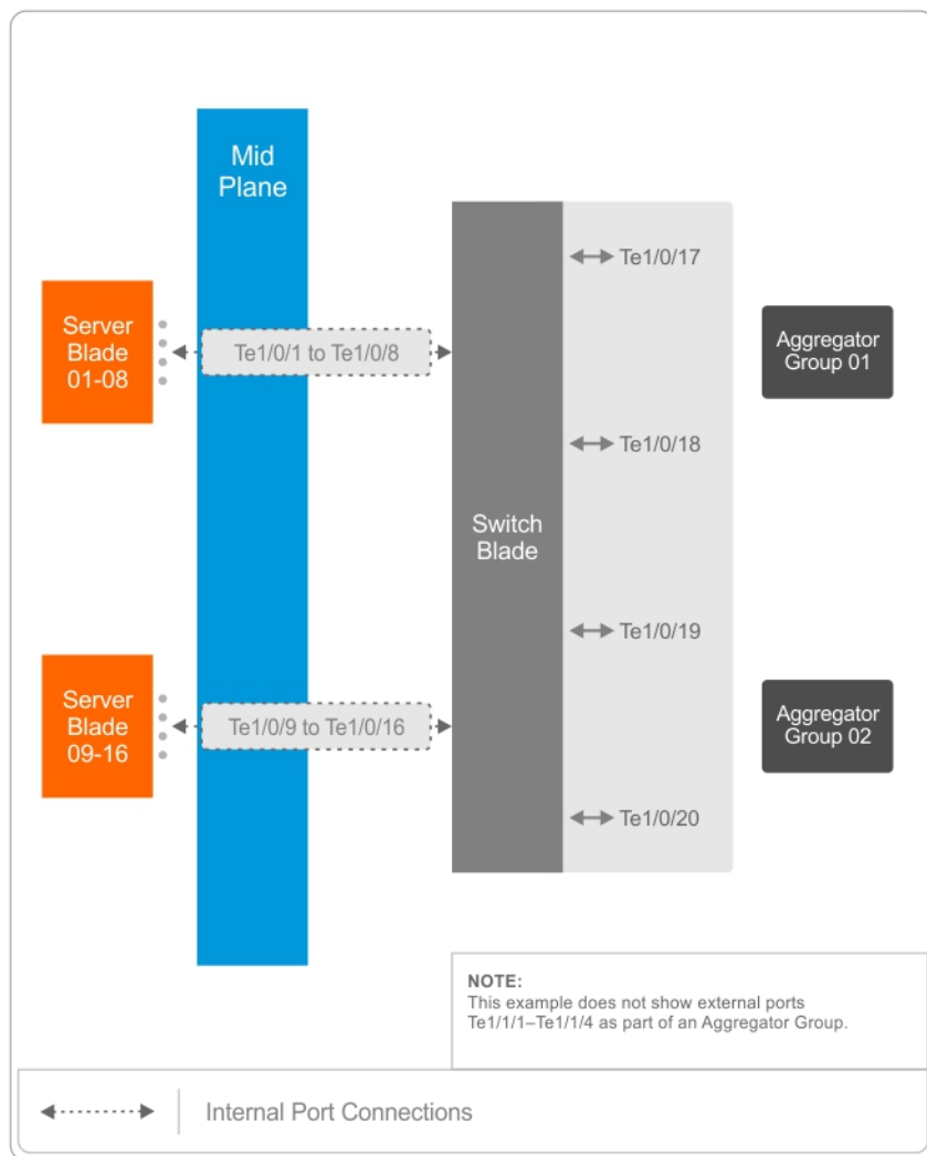
Figure 8. Single M8024K Switch Configuration with Two Aggregator Groups
