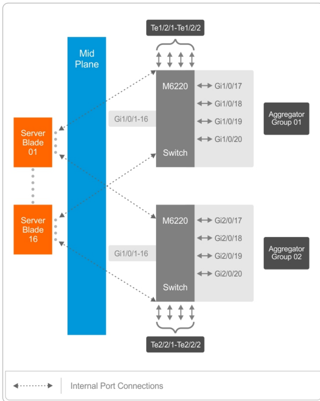
Figure 3. Default Aggregator Groups of a Stack of Two M6220 Switches
