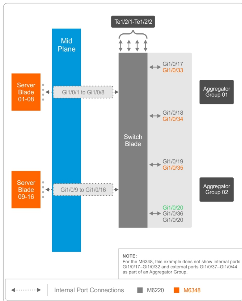
Figure 7. Single M6220/M6348 Switch Configuration with Two Aggregator Groups
