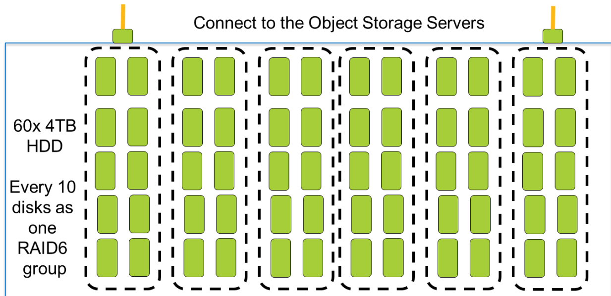
Figure 8: RAID6 Layout on MD3460 or MD3060e arrays
