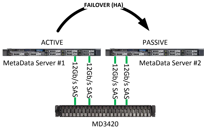
Figure 5: Metadata Server Pair
