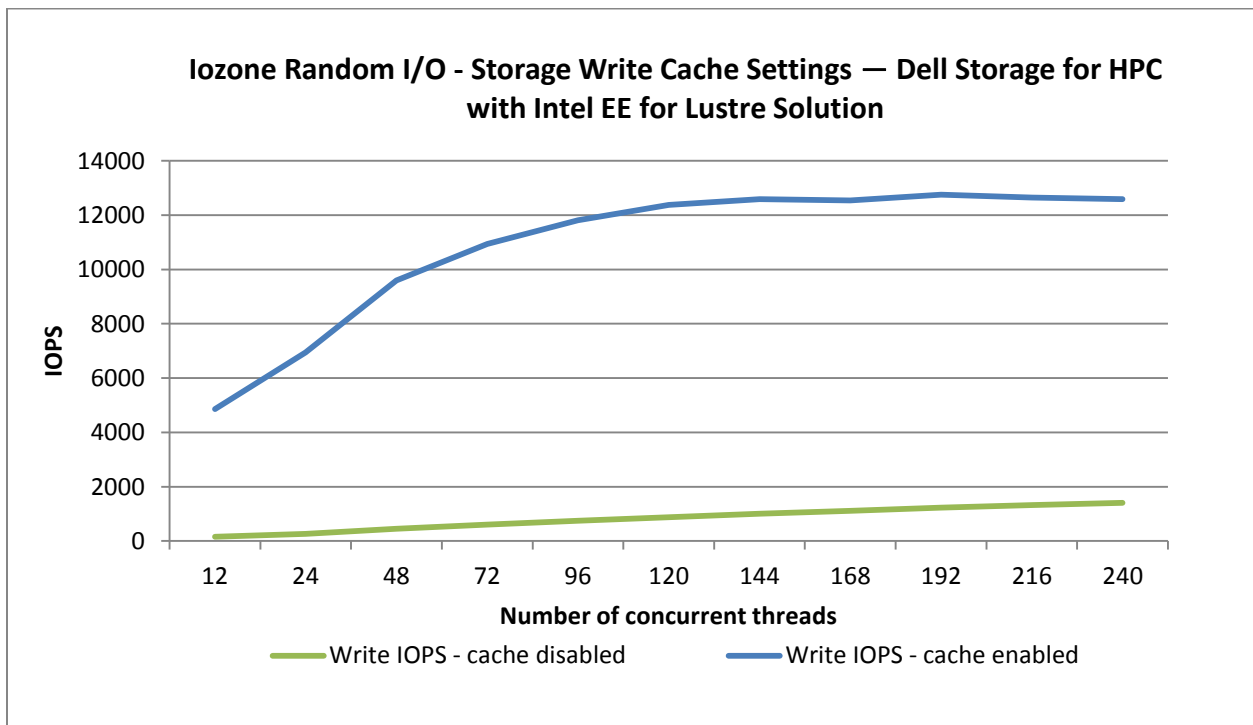
Figure 14: Write cache effect Random Write
