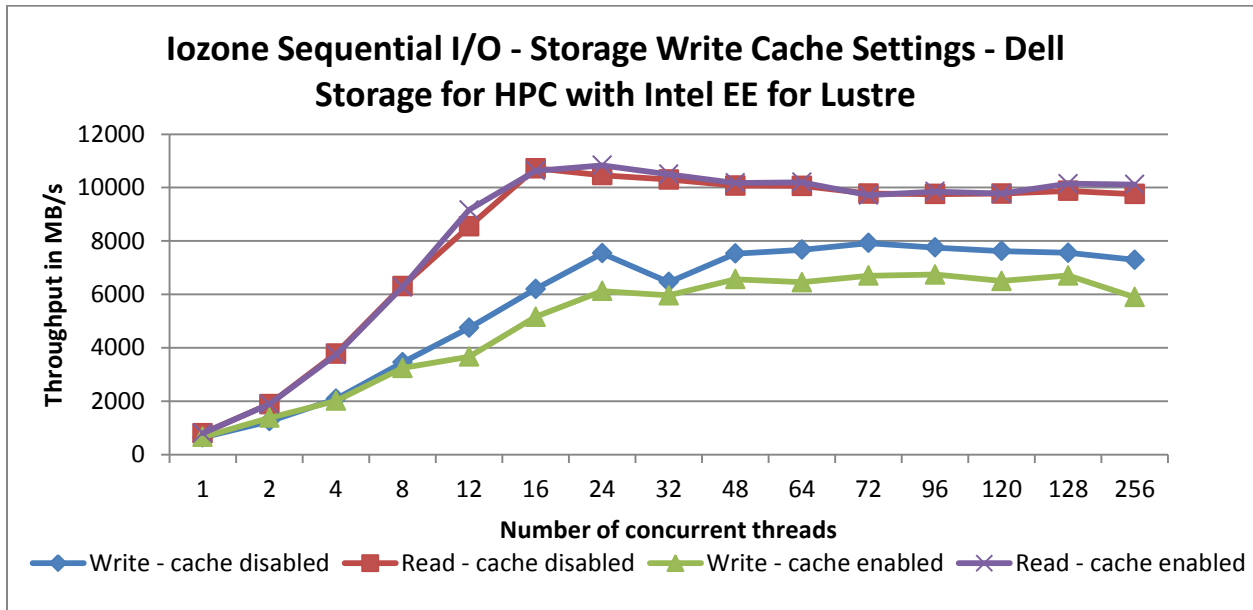
Figure 13: Storage Write Caching
