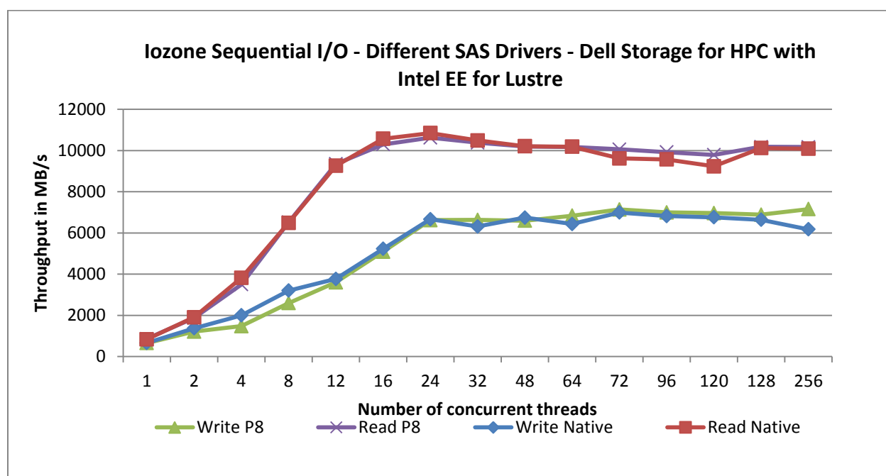
Figure 12: SAS drivers
