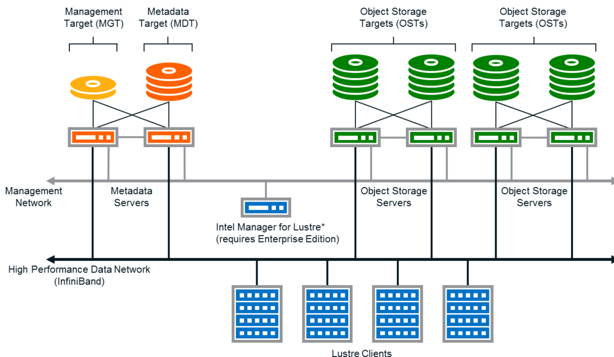
Figure 9: OSS Scalability
