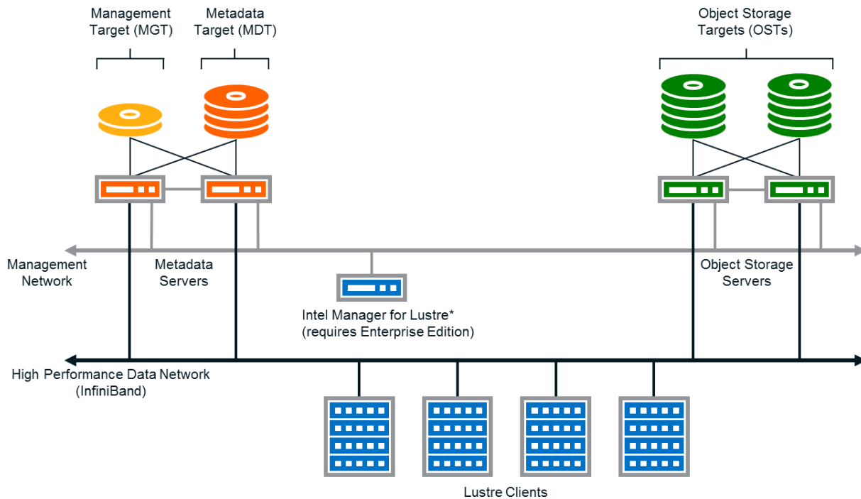
Figure 1: Lustre based storage solution components
