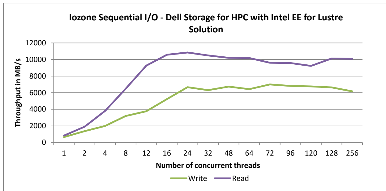
Figure 11: Sequential Reads / Writes Dell Storage for HPC with Intel EE for Lustre Solution
