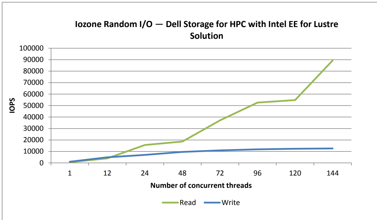
Figure 14: N-to-N Random reads and writes
