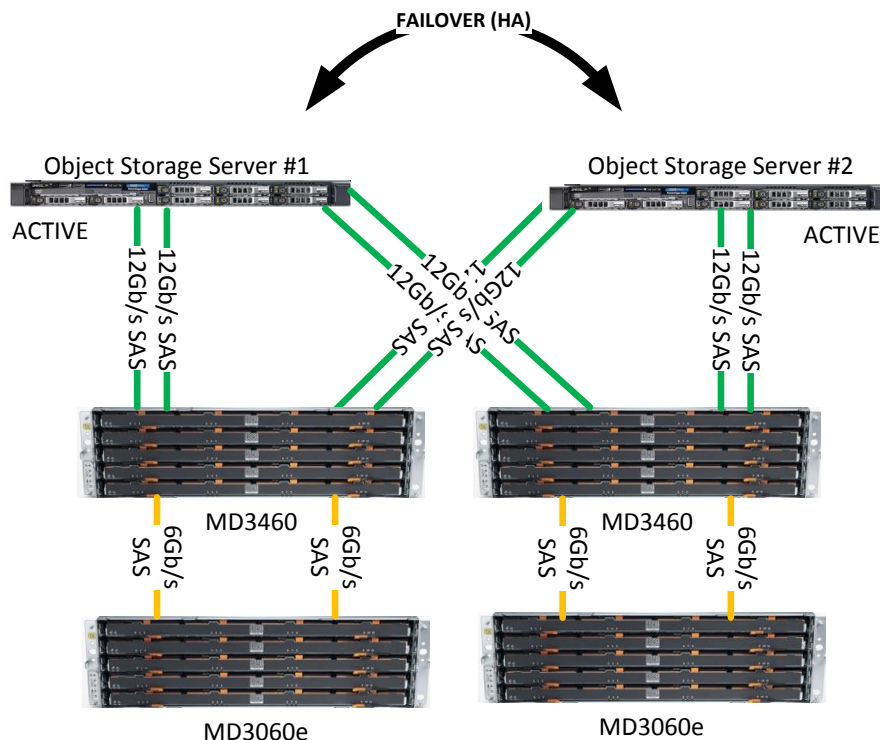
Figure 7: Object Storage Server Pair
