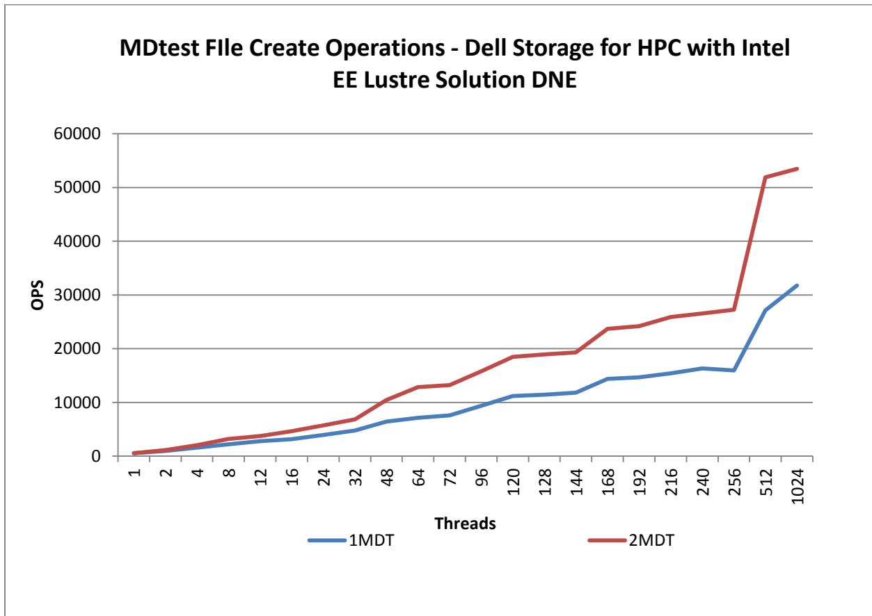
Figure 17: MDtest File Create Operations Lustre DNE
