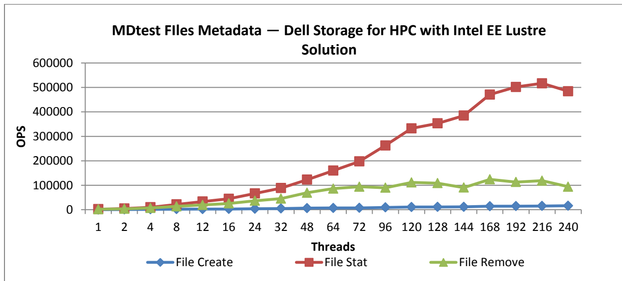
Figure 15: File Metadata Operations
