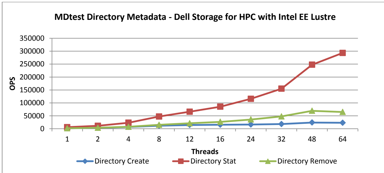
Figure 16: Directory Metadata Operations
