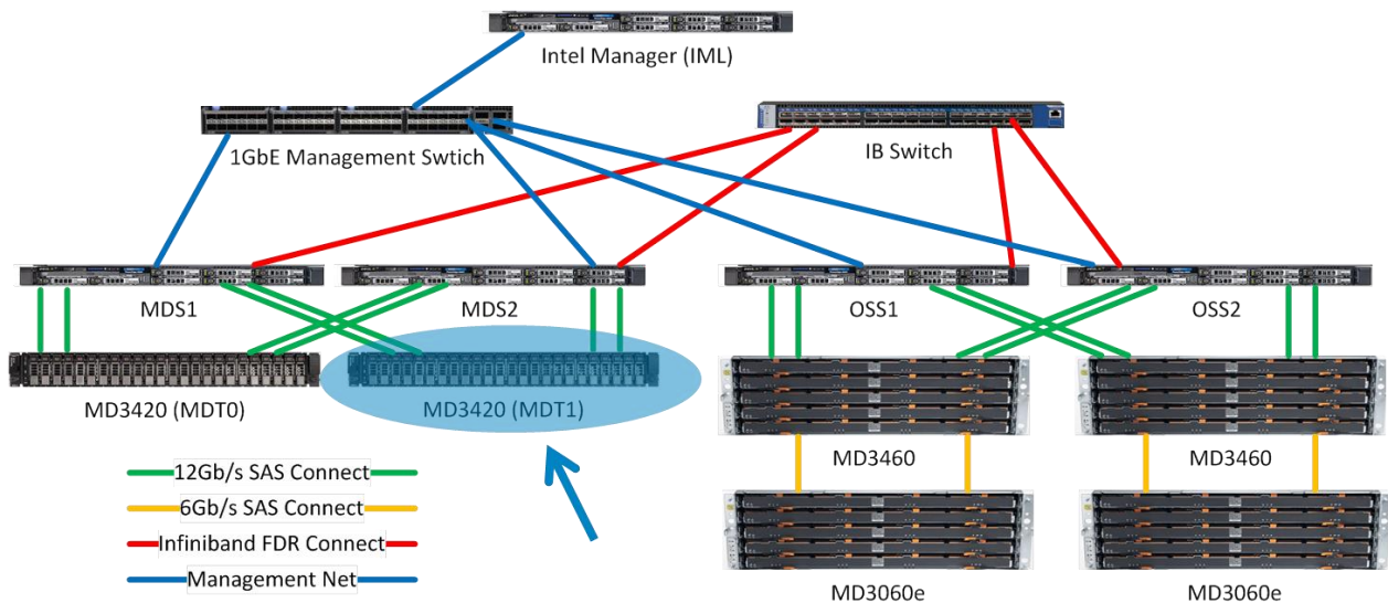
Figure 3: Lustre DNE option
