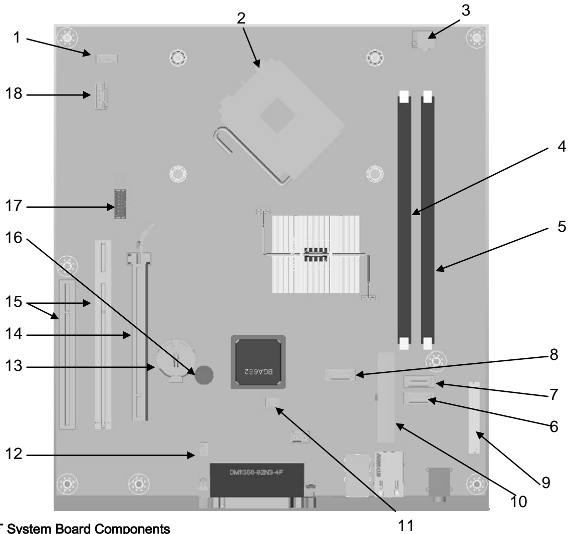
MT/DT System Board Components
